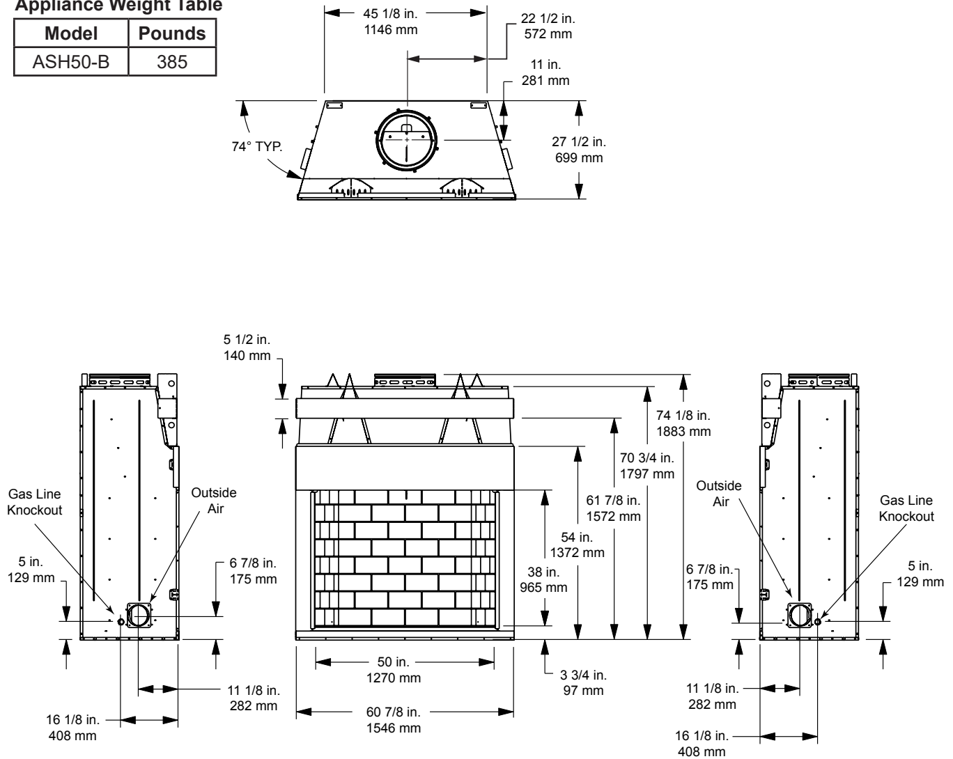
Figure 3.1 Appliance Dimensions
