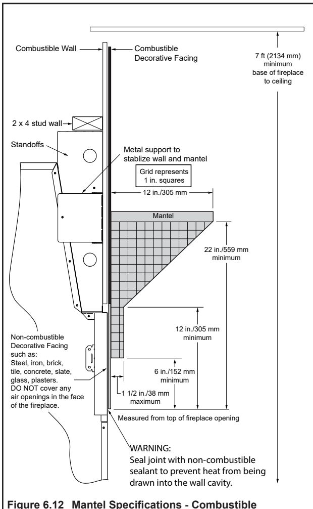
Figure 6.12 Mantel Specifications - Combustible
