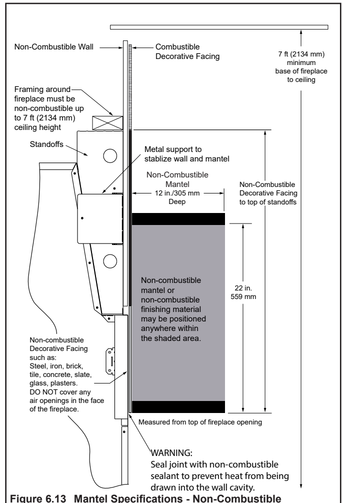
Figure 6.13 Mantel Specifications - Non-Combustible
