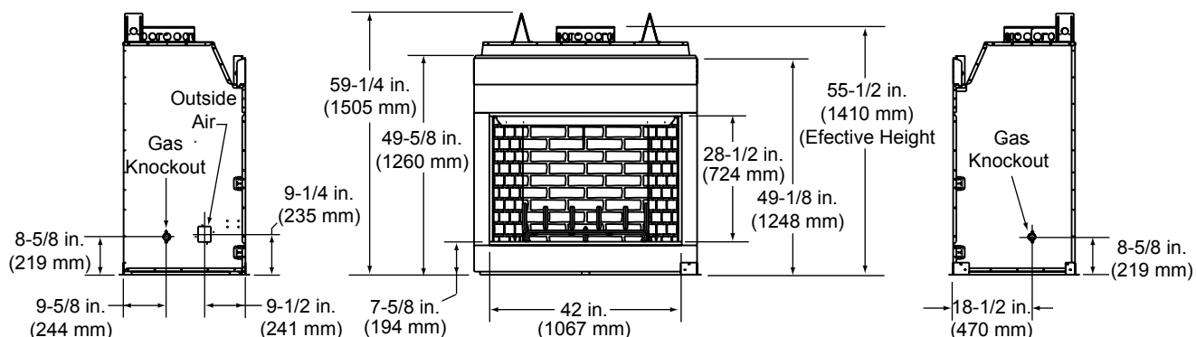
Figure 3.1 Appliance Dimensions
